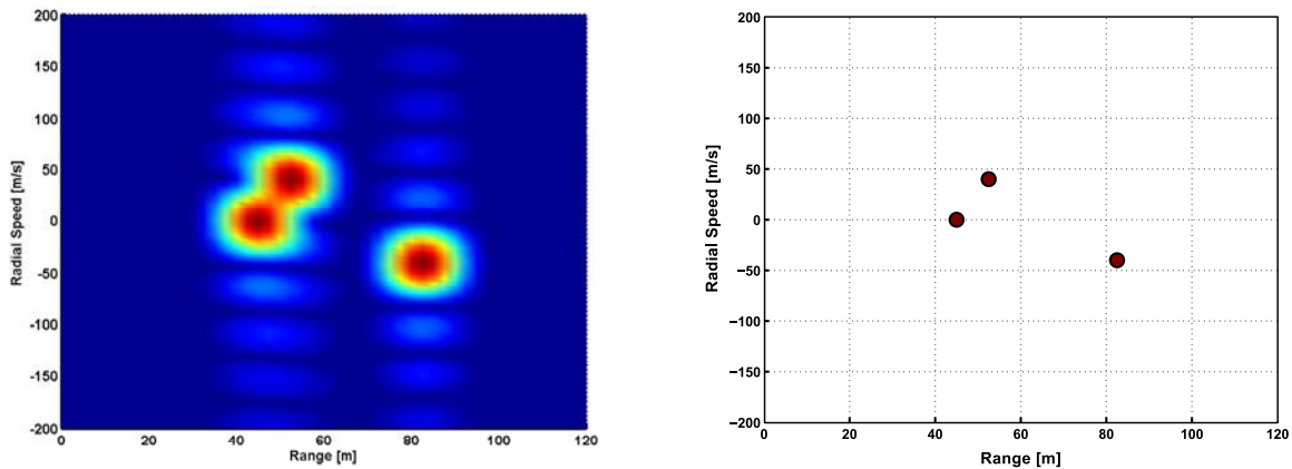
Figure 6: Simulation result with 3 targets and a signal-noise-ratio of 40 dB. Left diagram shows the range/velocity-plane reconstructed by the matched filter approach and right diagram shows the result obtained by CS.
