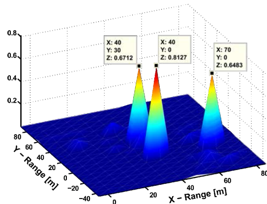
Figure 12: Reconstructed state vector using SGPL1 and with L = 800 from each tx-rx-pair.
