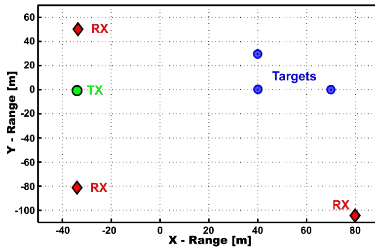
Figure 10: Simulation setup consisting of 1 transmitter (TX), 3 receivers (RX), and 3 targets.
