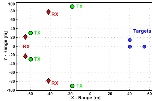
Figure 14: Simulation setup consisting of 4 TX, 4 RX, and 3 targets.
