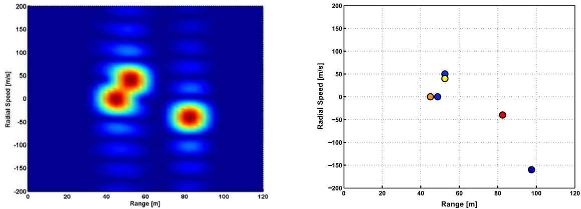
Figure 7: Same simulation as in the previous Fig. 6 however SNR is now 5 dB. Left diagram shows the range/velocity-plane reconstructed by the matched filter approach and right diagram shows the result obtained by CS.
