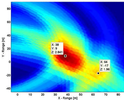
Figure 11: Target positions estimated by the matched filter approach.
