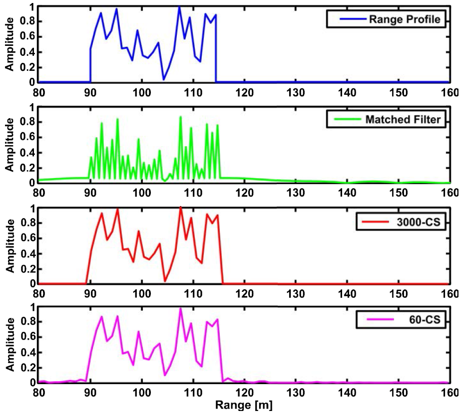
Figure 1: Pulse compression in the time domain with the matched filter approach and compressive sensing.
