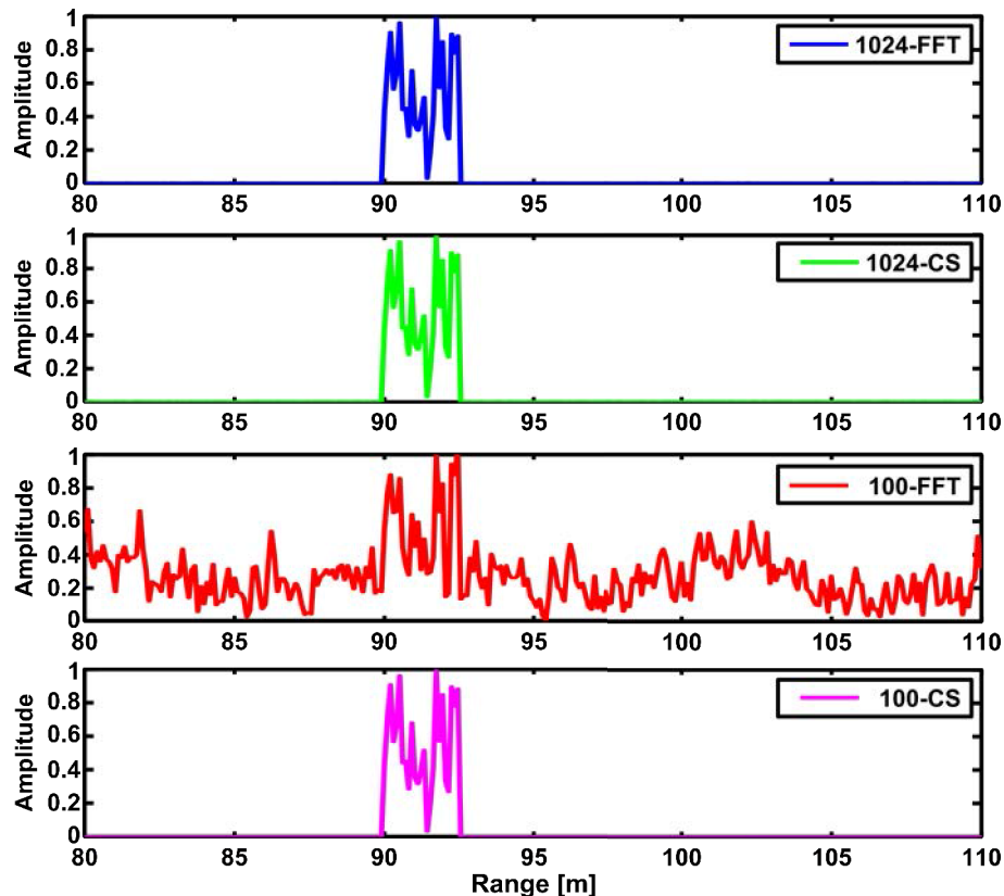
Figure 2: Comparison between traditional pulse compression (matched filter) and CS for various number of measurement samples.
