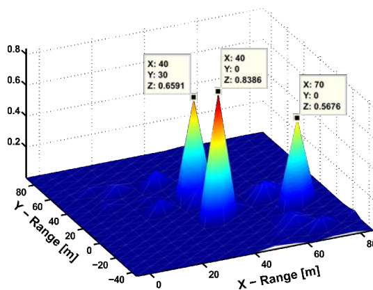
Figure 13: Target state vector obtained by SGPL1 and L = 50 samples from each tx-rx-pair.
