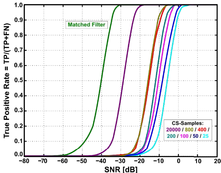
Figure 17: True target position rate versus Signal-Noise-Ratio for different number of samples L .
