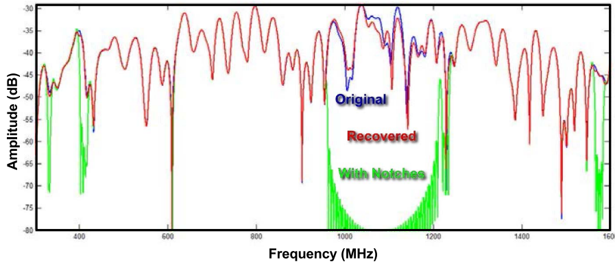
Figure 3: Recover of a signal with spectral gaps using CS (courtesy by Nguyen, CoSeRa 2012, [25]).
