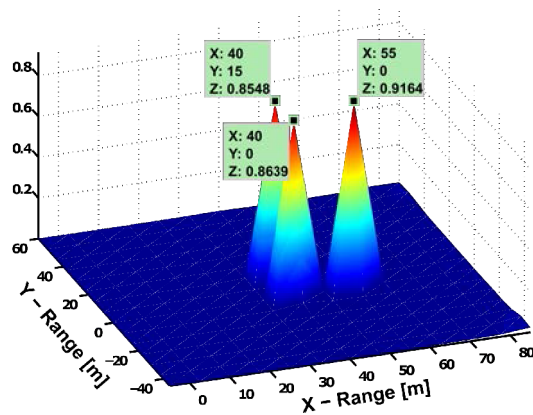
Figure 16: Target state vector obtained by SGPL1 and L = 50 samples from each tx-rx-pair.
